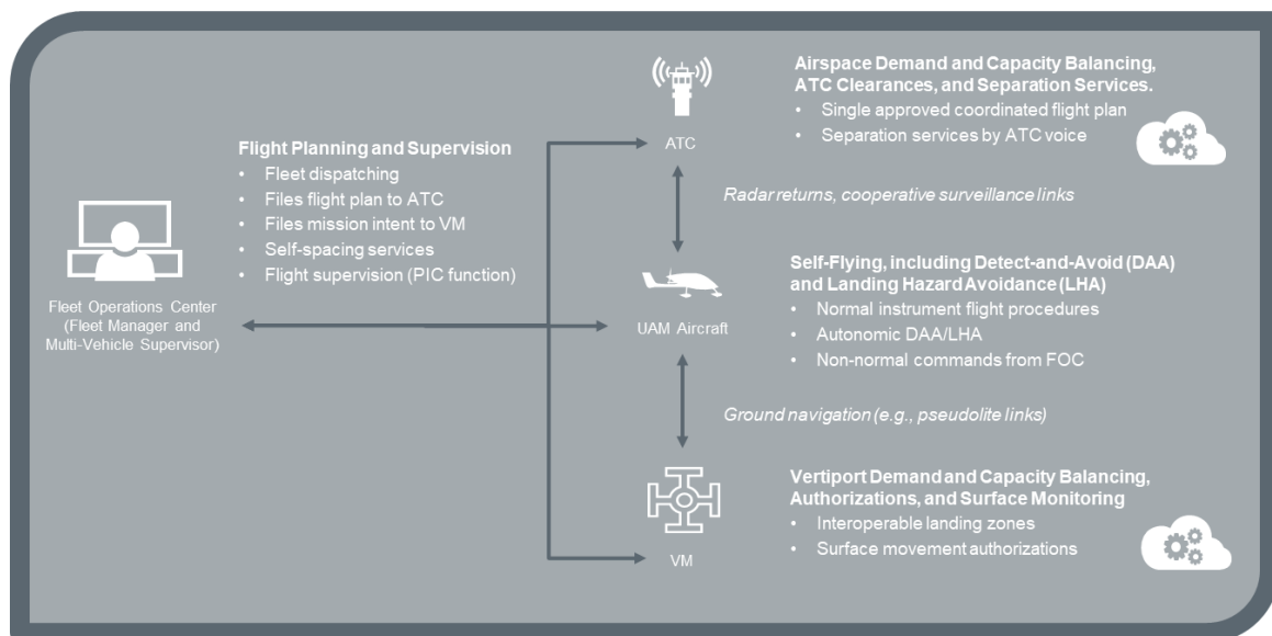
Figure 11. UAM System Functions with Embedded Enabling Capabilities
